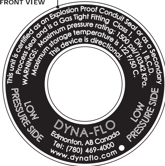
METAL TAG FRONT VIEW
