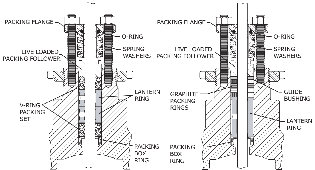
TYPICAL LIVE LOADED PACKING WITH PTFE V-RING PACKING SETS
