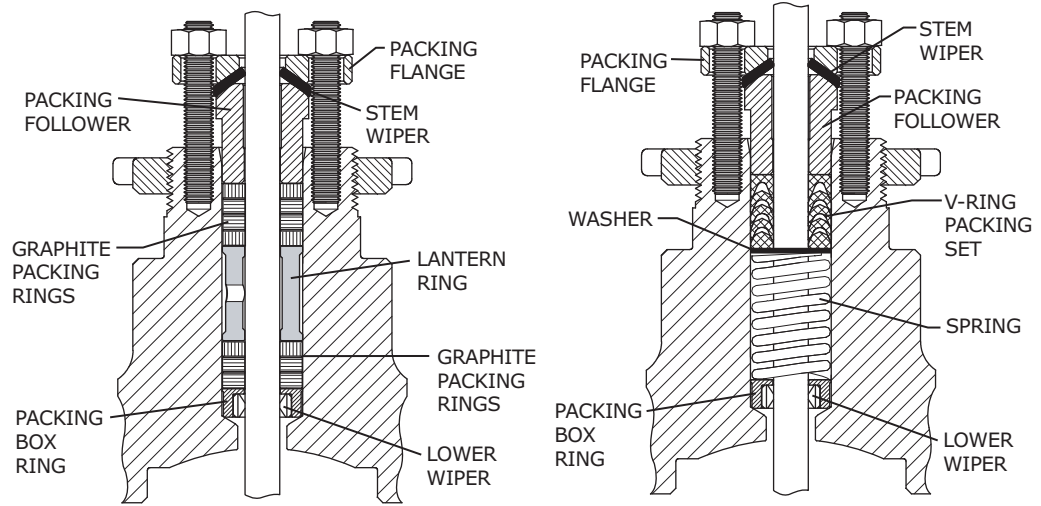
STANDARD HIGH TEMPERATURE PACKING DIAGRAM
